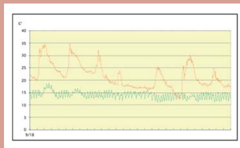
Temperature stability
